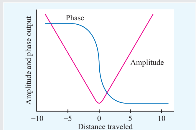
Figure TF11-2 Amplitude and phase responses as a function of the distance by which the magnetic core is moved away from the center position.
