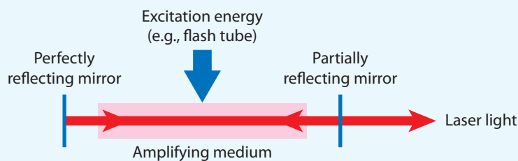
Figure TF15-3 Laser schematic.
