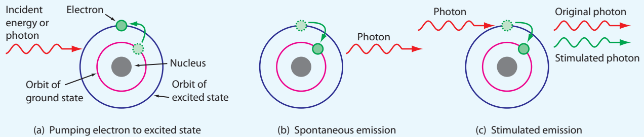
Figure TF15-2 Electron excitation and photon emission.
