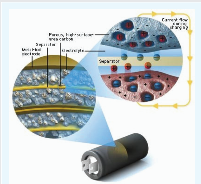
Figure TF8-1 Cross-sectional view of an electrochemical double-layer capacitor (EDLC), otherwise known as a supercapacitor. (Courtesy of Ultracapacitor.org.)
